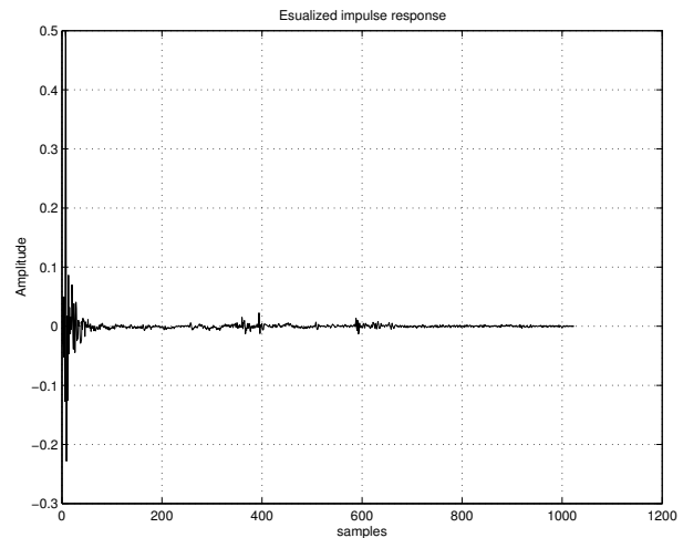
Figure 23. Direct front equalized impulse response.
