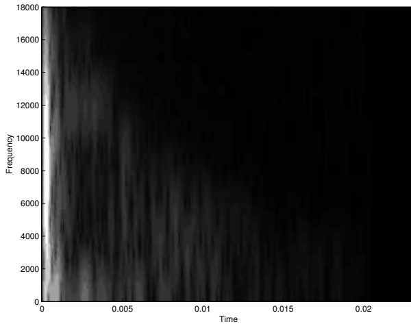
Figure 30. S-FDTW impulse response spectrogram
