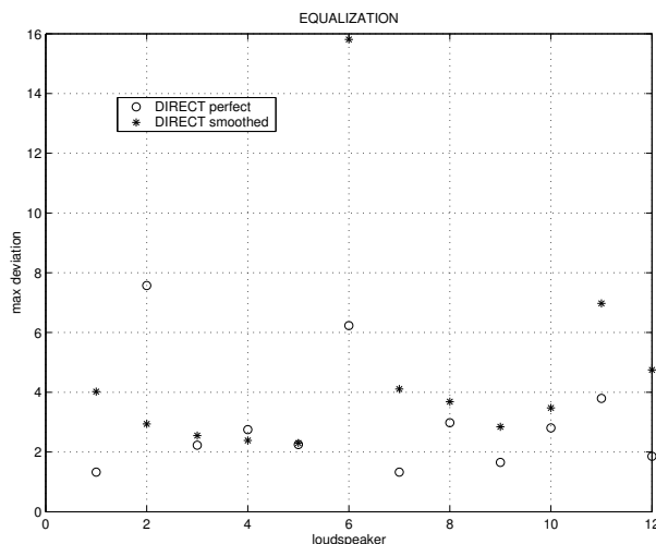
Figure 22. Jmax for room equalization
