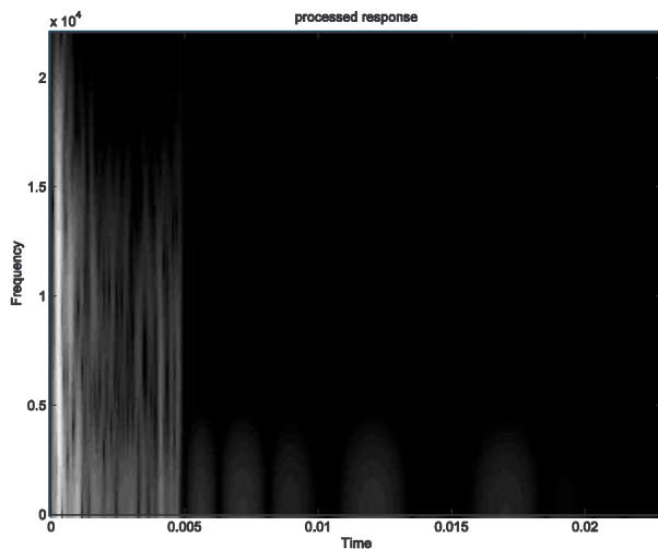
Figure 28. H-FDTW impulse response spectrogram
