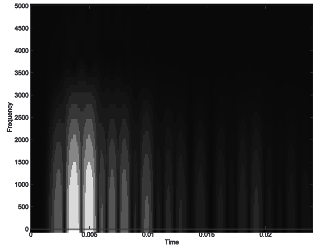
Figure 26. Direct front equalized low-passed impulse response spectrogram
