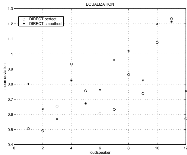
Figure 19. J for electronic equalization
