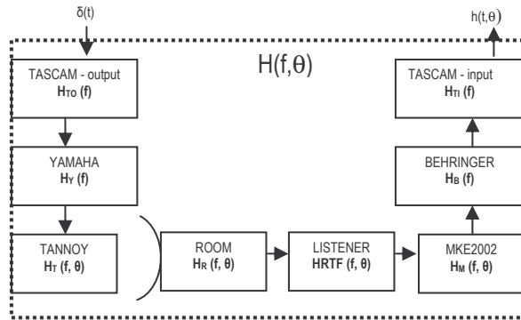
Figure 16. Electro-acoustic chain
