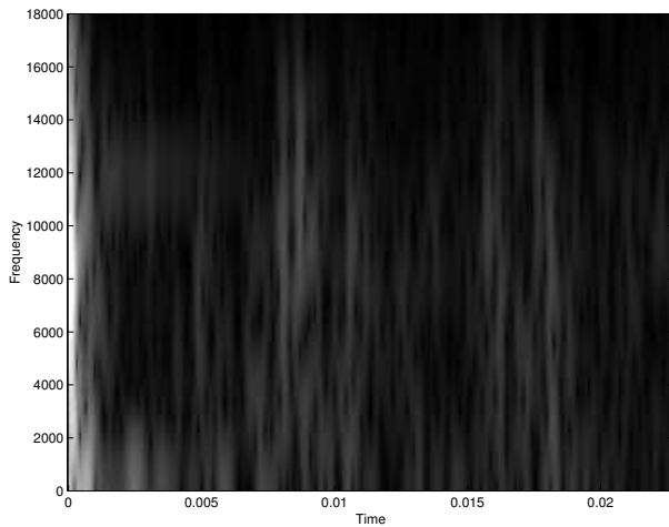
Figure 24. Direct front equalized impulse response spectrogram
