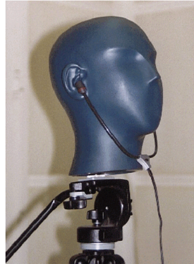
Figure 14. MKE2002 microphone
