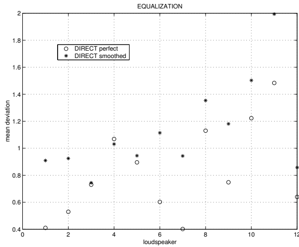
Figure 21. J for room equalization
