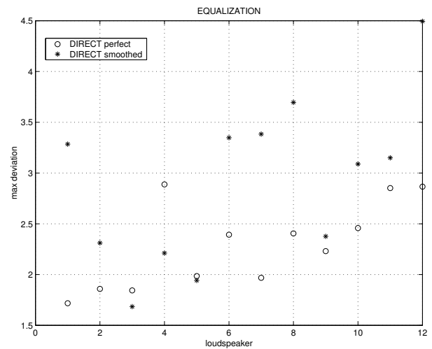
Figure 20. J max for electroacoustic equalization
