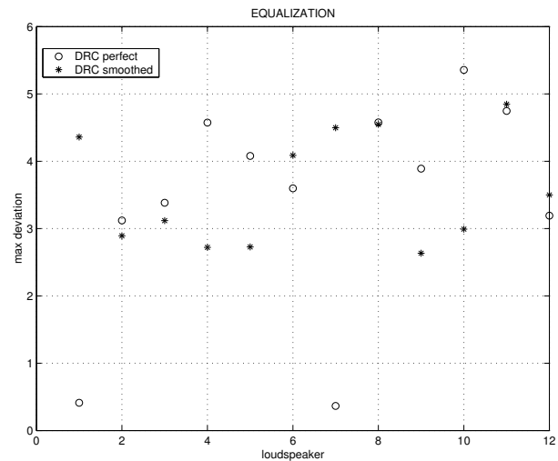
Figure 18. J max for electroacoustic equalization
