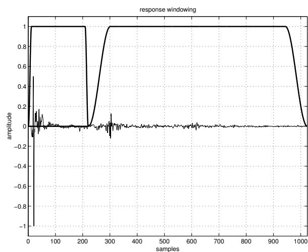
Figure 27. Frequency dependent hard time windowing
