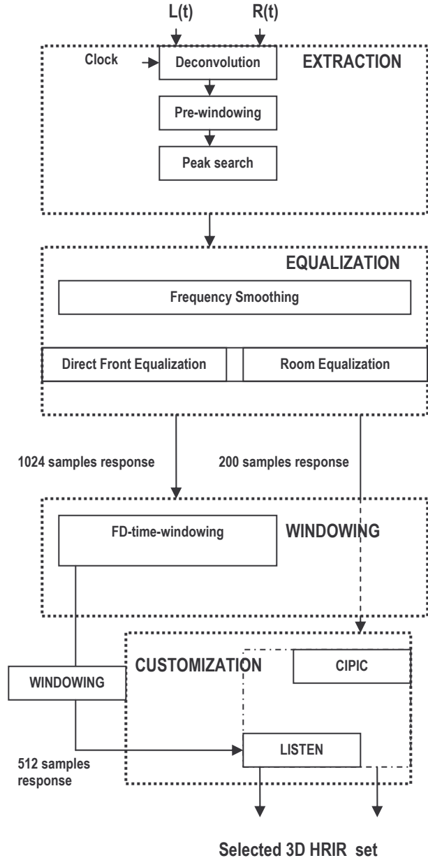
Figure 15. Processing chain
