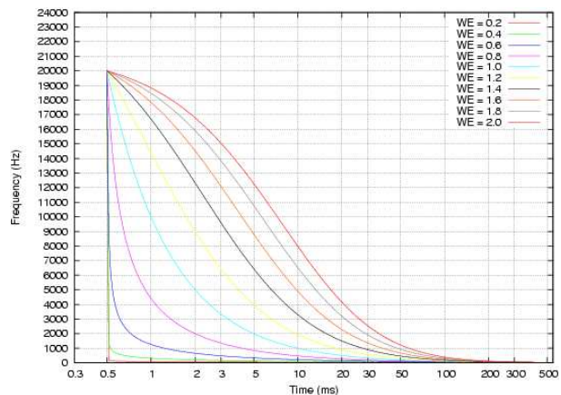
Figure 29. Window exponent for fdtw
