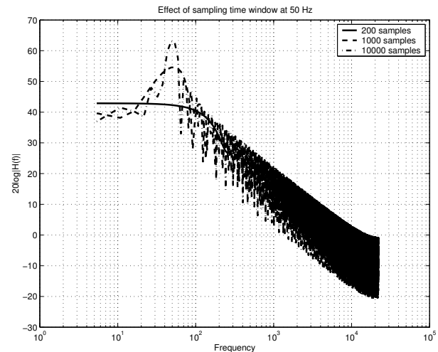
Figure 1. Sampling window effect at 50 Hz
