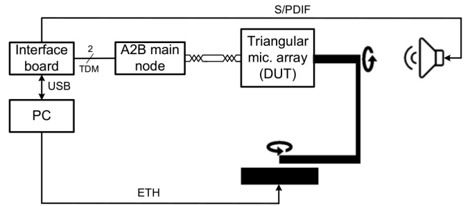
Fig. 9. Experimental measurement setup.
