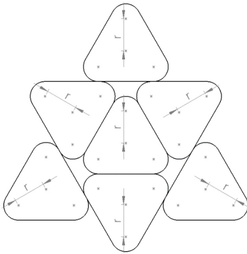
Fig. 11. Design of a meta-array with seven triangular arrays and 28 capsules.
